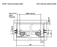
Installation dimensions
